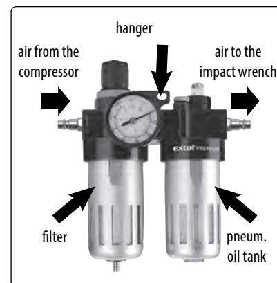
Fig. 10, description of the Extol® 8865105 Treatment unit
